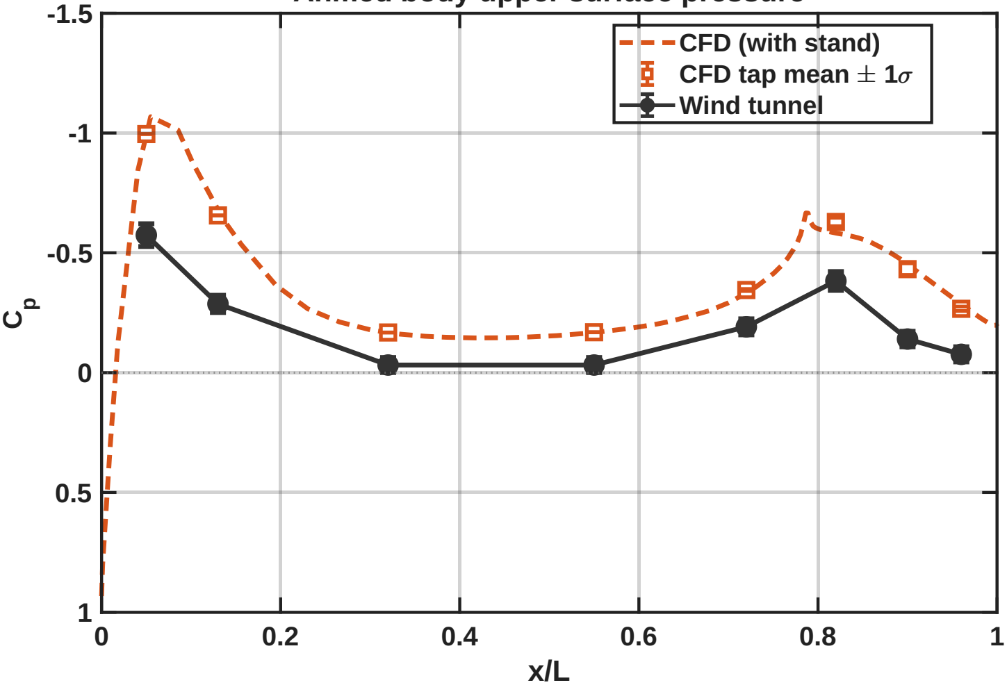
Ahmed body upper surface pressure
